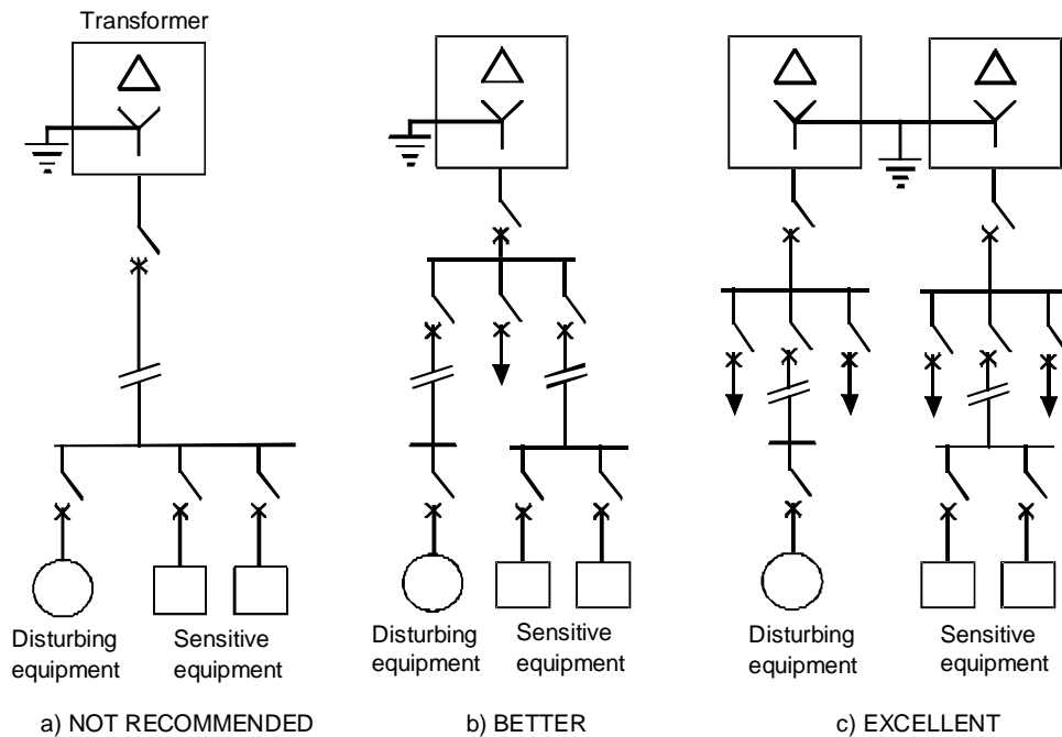
Figure 3 - Segregation of the electricity distribution for different applications
