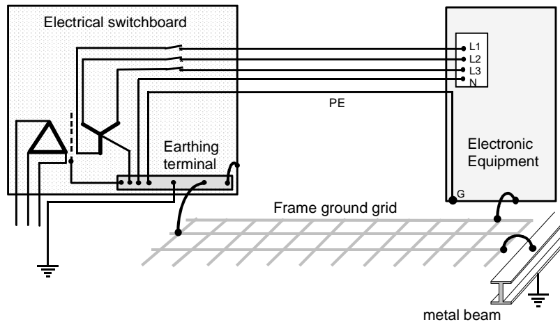
Figure 19 - Mesh BN example
