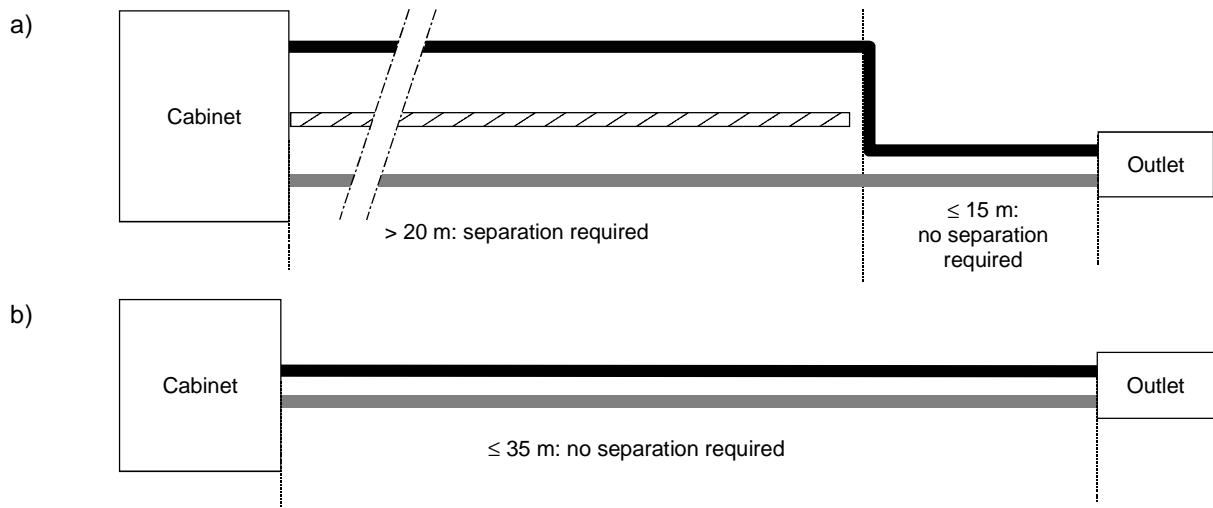
Figure 5 - Separation between power and data cables
