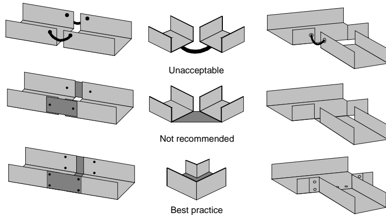
Figure 11 - Continuity of metallic system components
