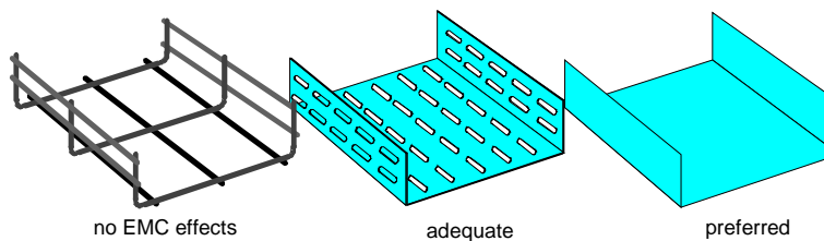
Figure 9 - EMC ranking for different metallic trays
