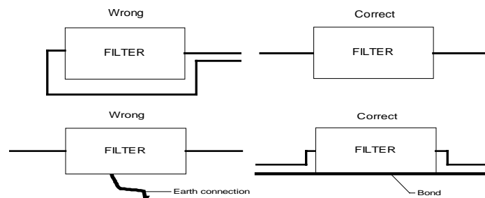
Figure 23 - Earthing and bonding of filters
