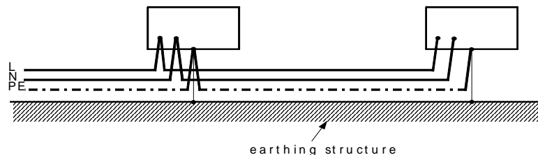
Figure 27 - Earthing arrangement
