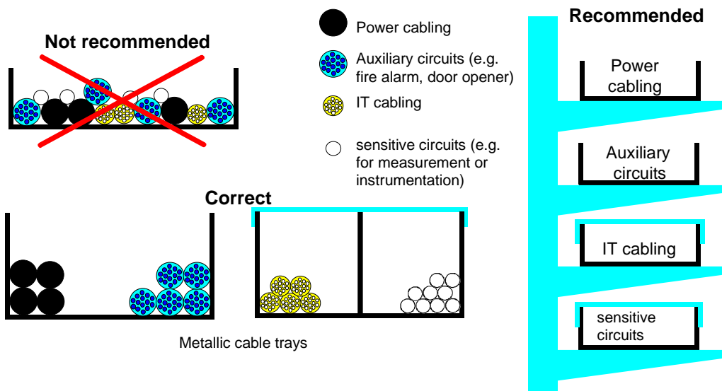
Figure 8 - Separation of cables in cable management systems
