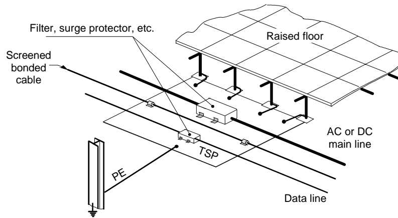
Figure 22 - Example of transient suppressing plate installation details
