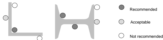
Figure 12 - Location of cables inside metallic construction elements
