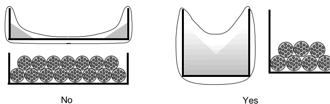
Figure 10 - Cable arrangement in a metallic section
