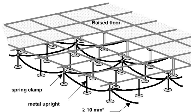
Figure 21 - Raised floor
