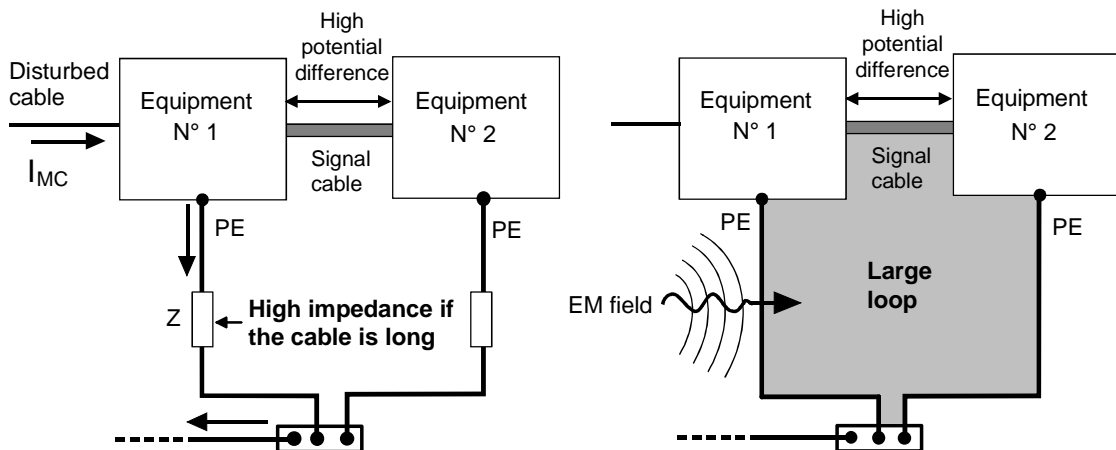
Figure 15 - Example of high common impedance and large loop
