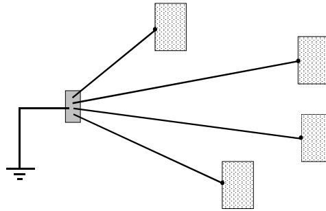
Figure 14 - IBN (star network)
