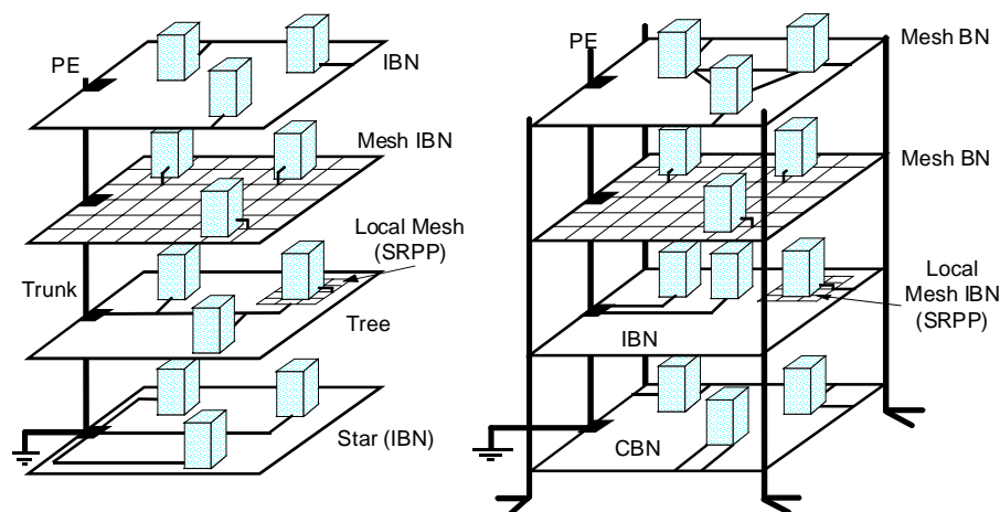
Figure 18 - Examples of bonding networks
