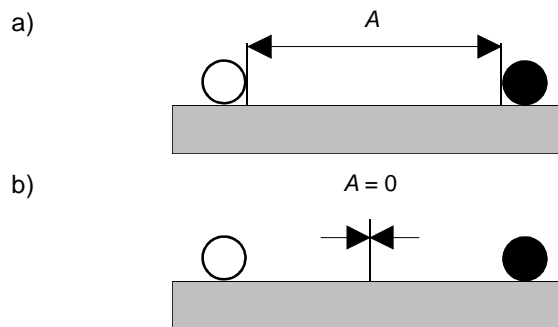
Figure 6 - Examples of power cables and information technology cables that run parallel without divider
