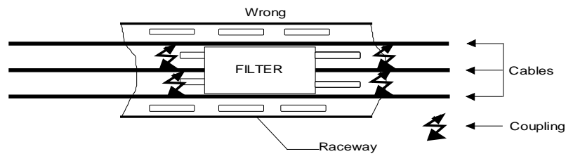
Figure 24 - Mounting of filters
