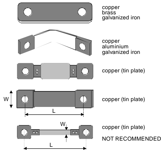
Figure 20 - Example of bonding straps
