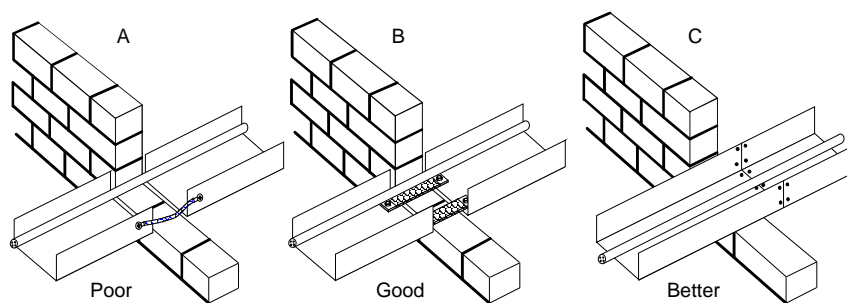
Figure 13 - Interruption of metallic sections
