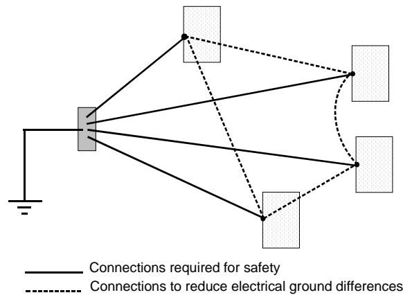
Figure 17 - Improvement of star earthing network
