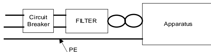
Figure 25 - Installation of power filter
