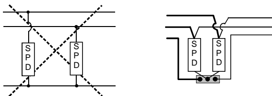
Figure 30 – Short connections of surge protective devices
